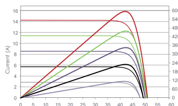
Current-Voltage & Power-Voltage Curves (600W)
