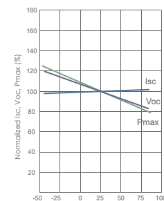
Temperature Dependence of Isc, Voc, Pmax
